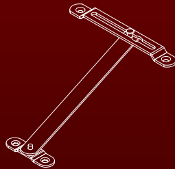
Restrictor and Cleaning Stay - 22 cm
