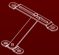
Restrictor and Cleaning Stay - 13 cm
