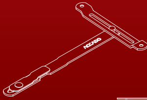
Espagnolette connected Restrictor and Cleaning Stay
